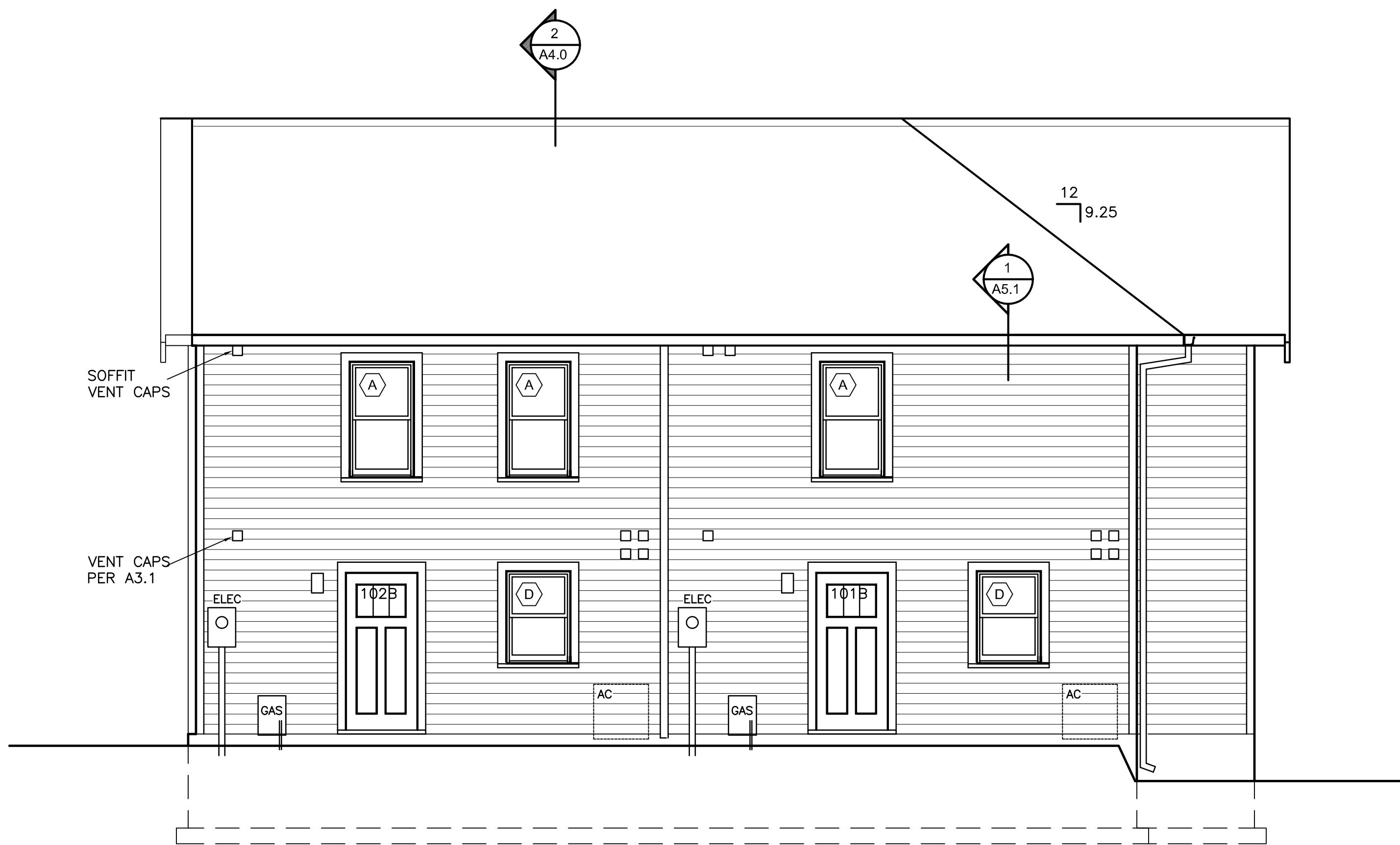
2 EAST ELEVATION A3.0 SCALE: 1/4"=1'-0"
