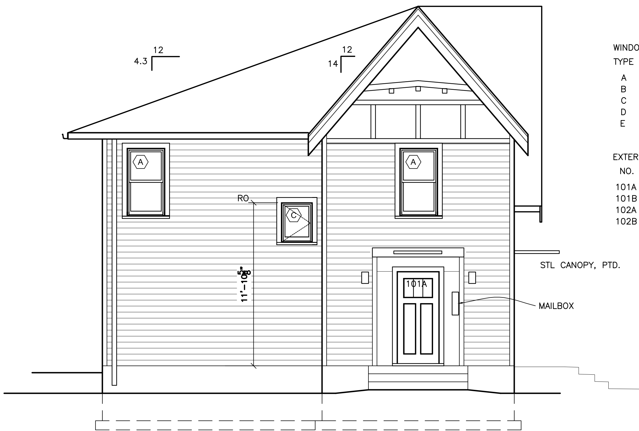
3 SOUTH ELEVATION A3.0 SCALE: 1/4"=1'-0"
