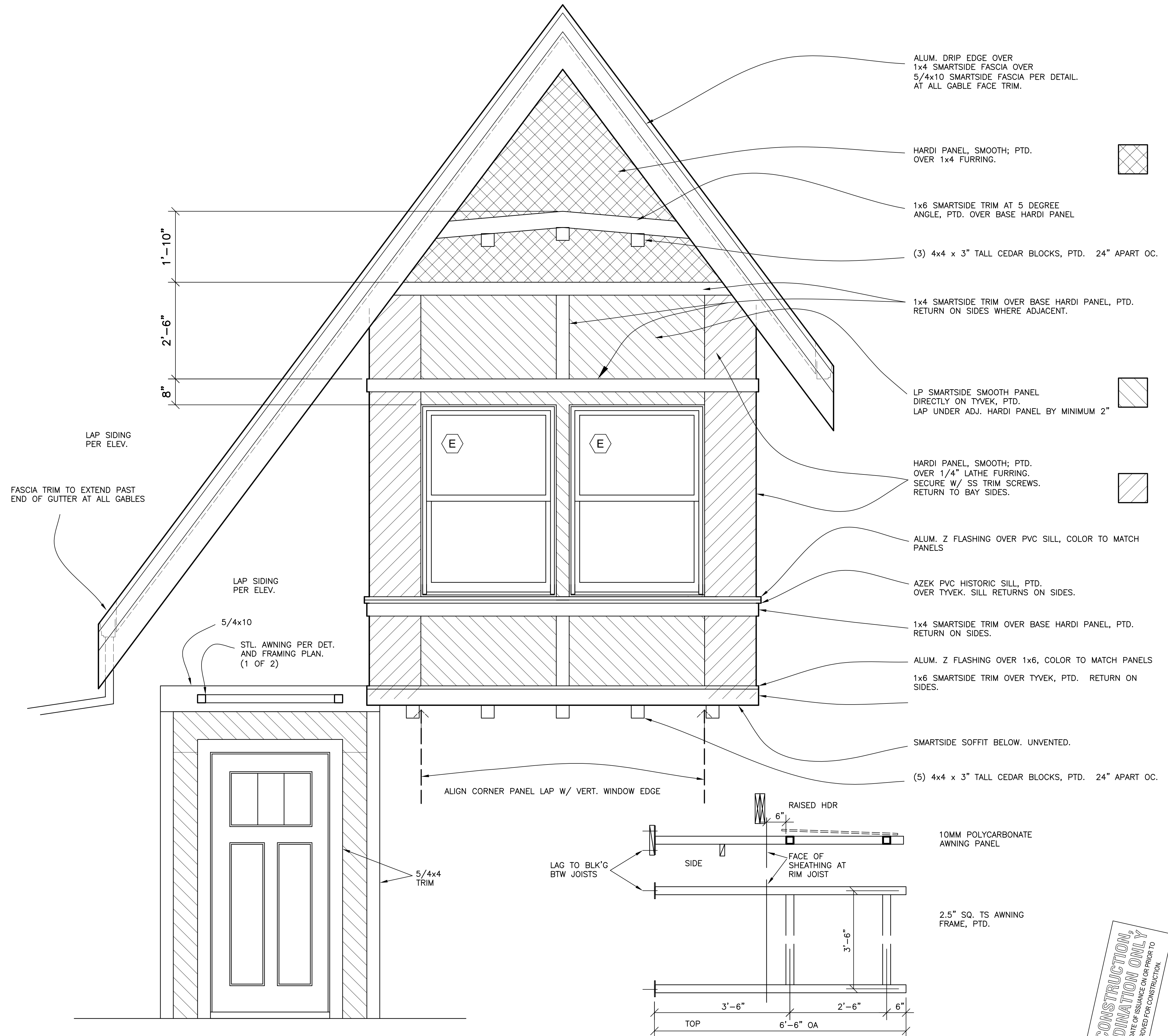
1 GABLE SIDING DETAIL A3.1 SCALE: 3/4"=1'-0"
