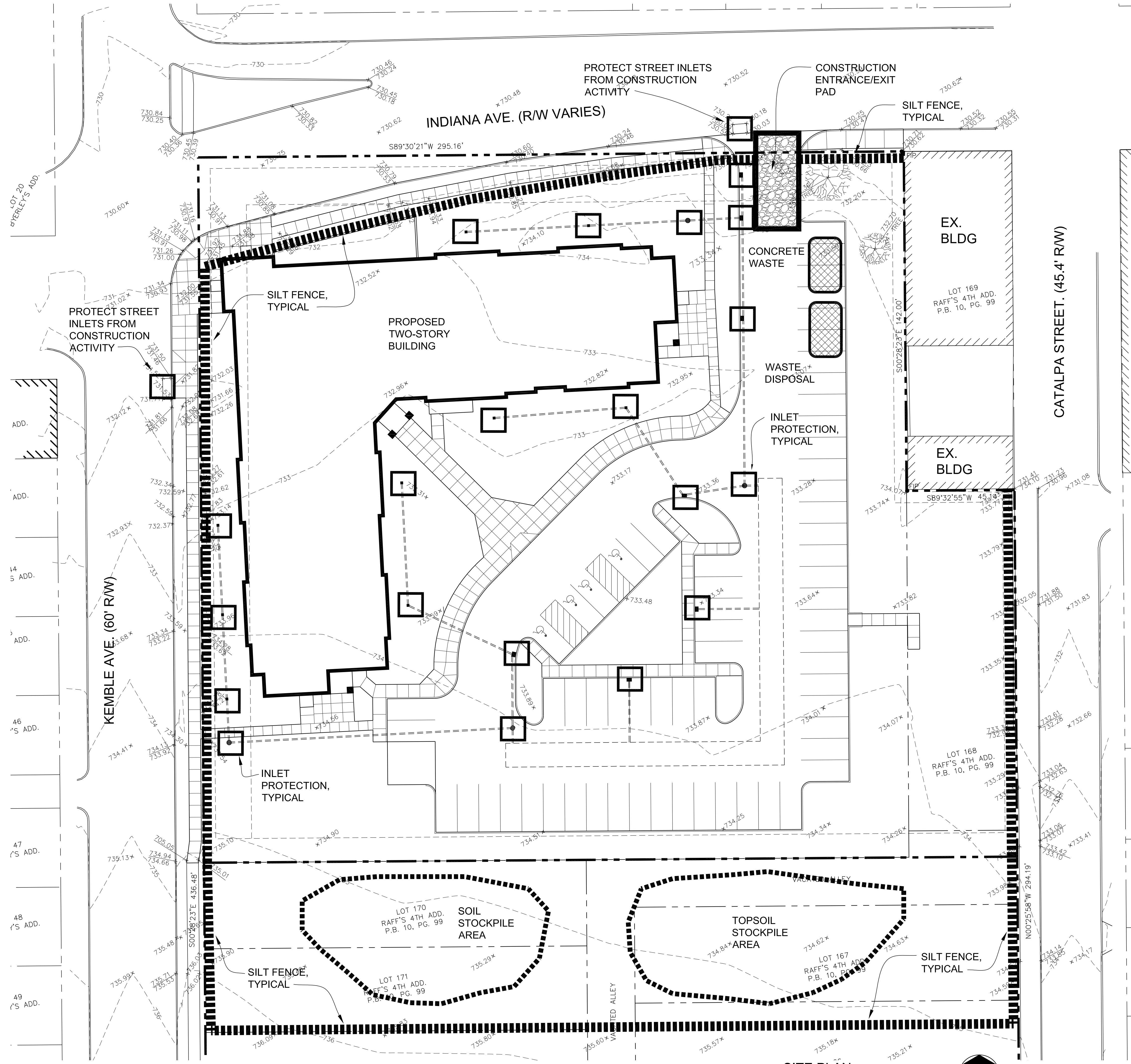
SITE PLAN 1" = 20'-0" NORTH
